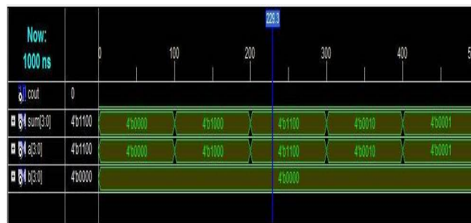
Fig.7 simulated result
