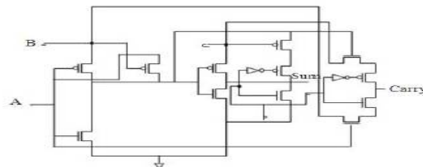
Fig.3 Full Adder
