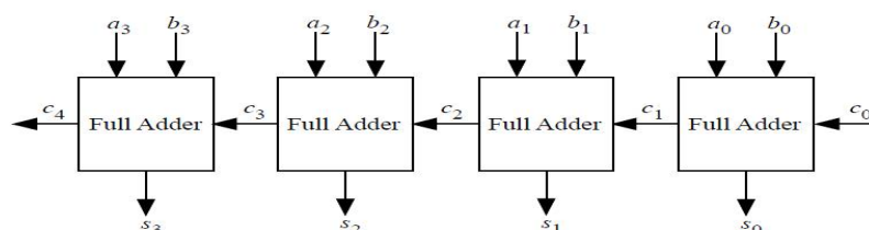
Fig.1 4-bit Ripple Carry Adder
