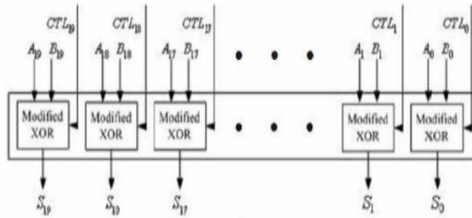
Fig.6. Carry free addition block
