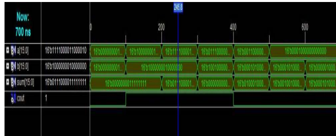
Fig.9.Simulated result
