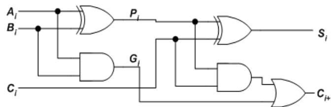
Fig.2 Carry-look-ahead-adder
