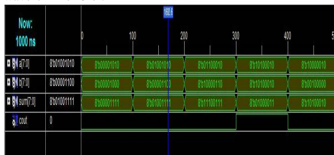
Fig.8 simulated result
