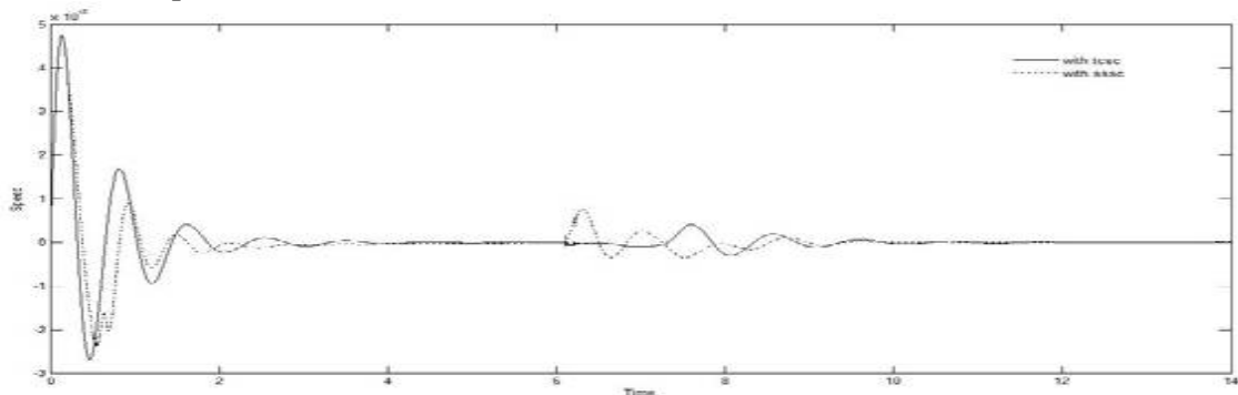
Fig 10 Comparison of Load angle with SSSC and with SVC a) Delta1-Delta3 b) Delta1-Delta2
