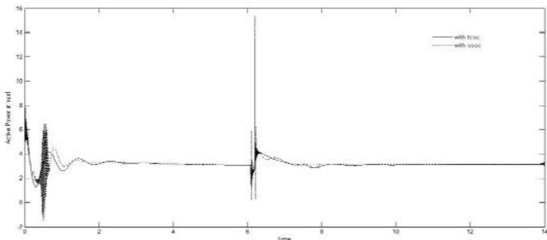
Fig 12 Comparison of active power at Bus 1 with SSSC and with TCSC
