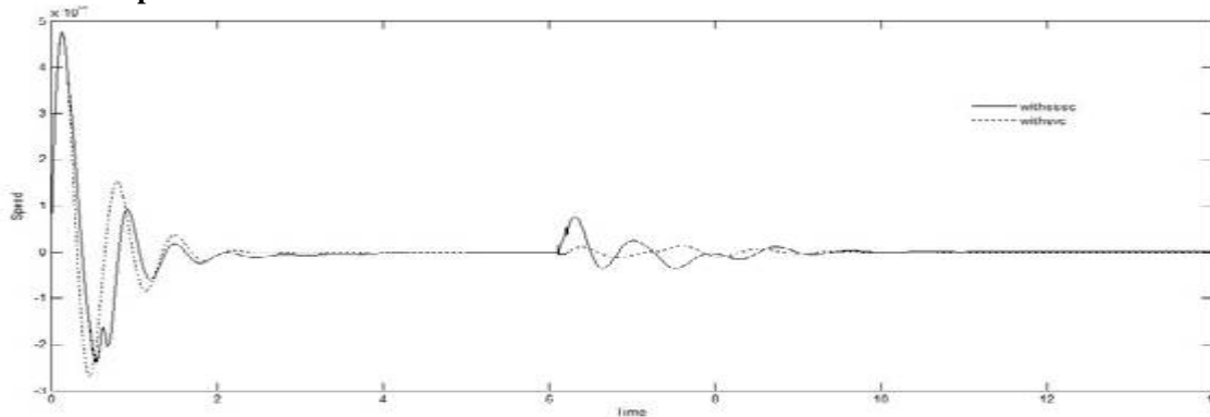
Fig 9 Comparison of speed(wm1-wm3) with SSSC and with SVC
