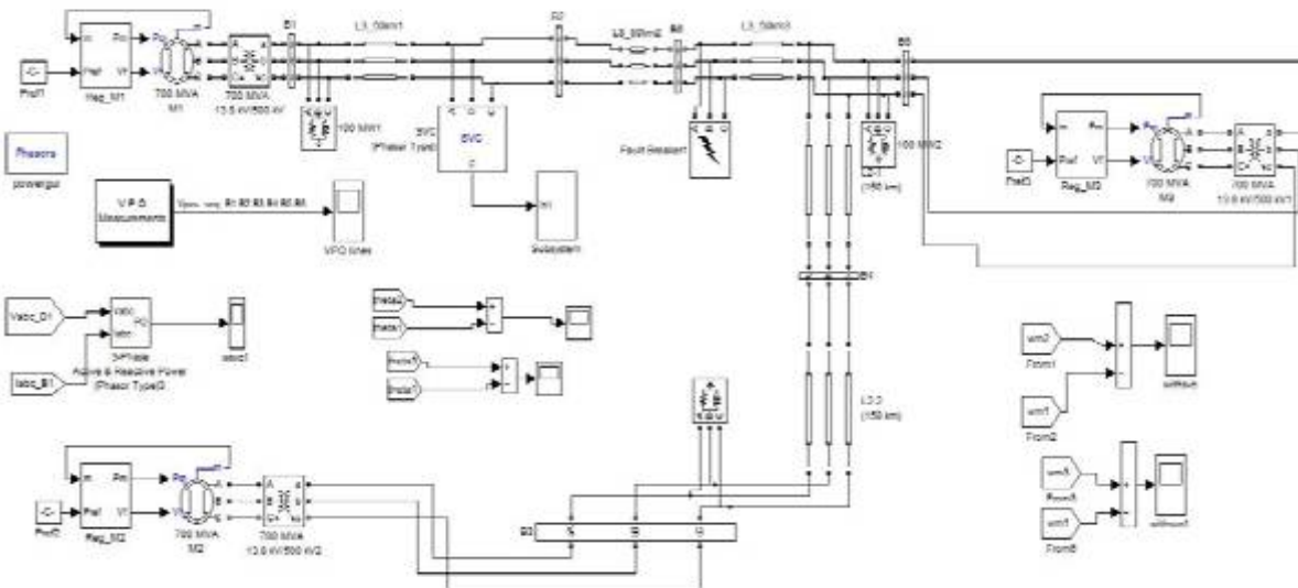
Fig 5 Simulink model with SVC
