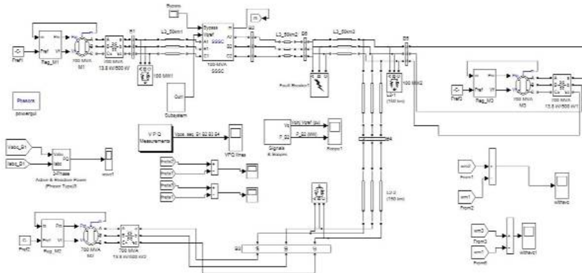
Fig 3 Simulink model with SSSC
