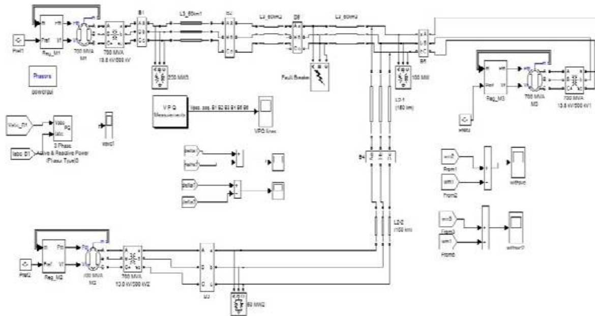
Fig 2. Simulink model of 3 machine 9 bus system
