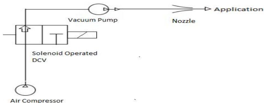
Fig 3: Pneumatic circuit for automatic seed sowing machine.
