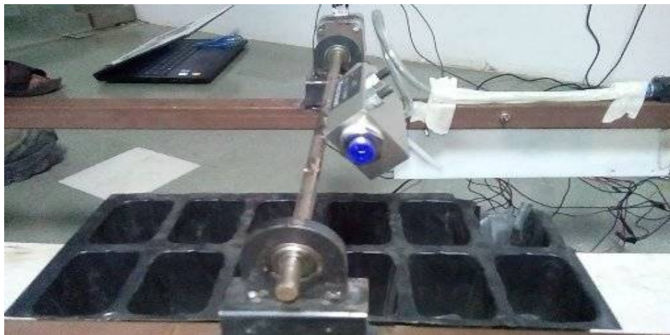
Fig 5: Actual Vacuum pump with pneumatic pipe and conveyor belt
