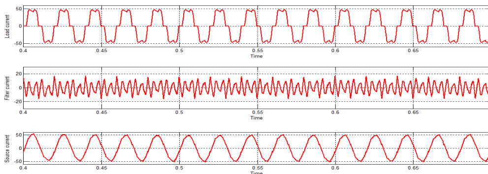
Fig:10 Wave forms of a) load current b) compensating current c) supply currents
