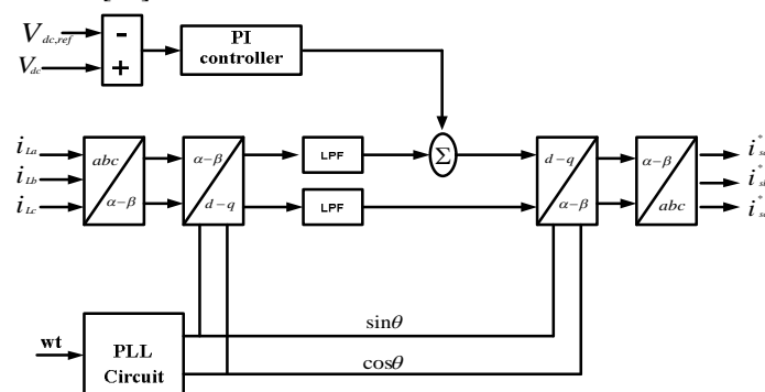
Fig 4: Control Diagram of SRF Theory
