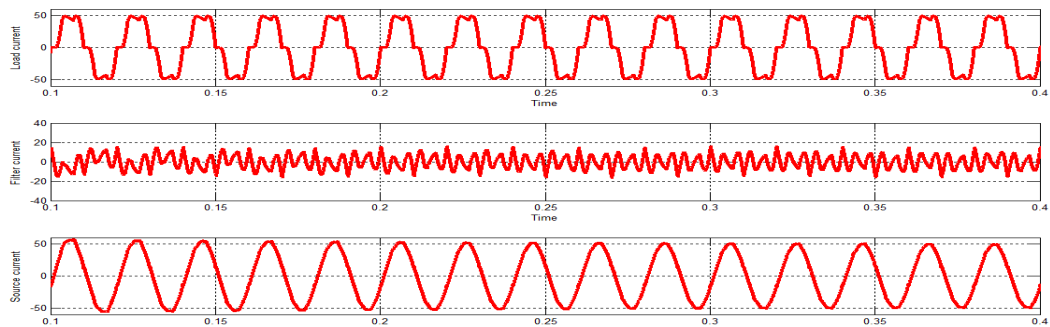
Fig:9 Wave forms of a) load current b) compensating current c) supply currents
