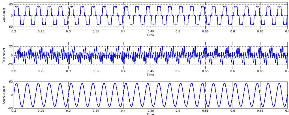
Fig:12 Wave forms of a) load current b) compensating current c) supply currents
