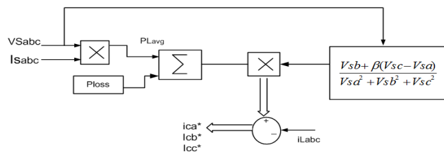
Fig 5: Control diagram of ISC Theory, phases a and c are identical as phase b
