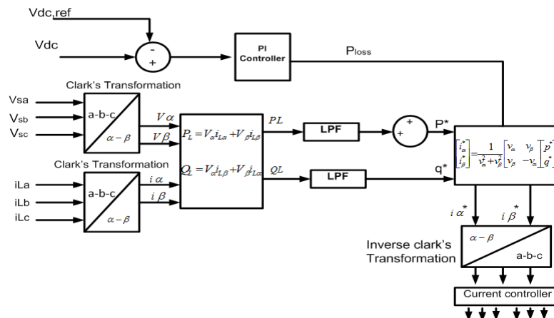
Fig 3: Control scheme using instantaneous P-Q Theory
