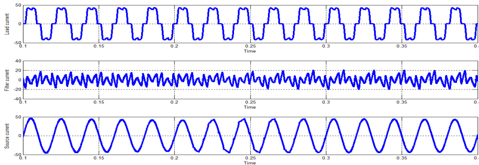
Fig 11: Wave forms of a) load current b) compensating current c) supply currents
