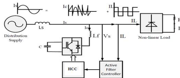
Fig. 1: Block Diagram of Shunt Active Power Filter.
