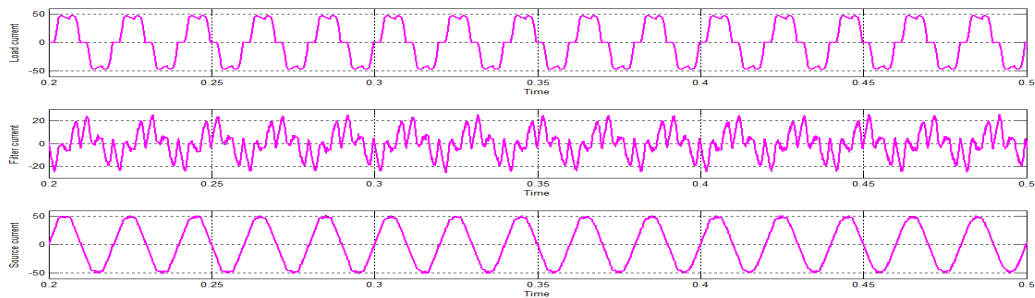
Fig:8 Wave forms of a) load current b) compensating current c) supply currents
