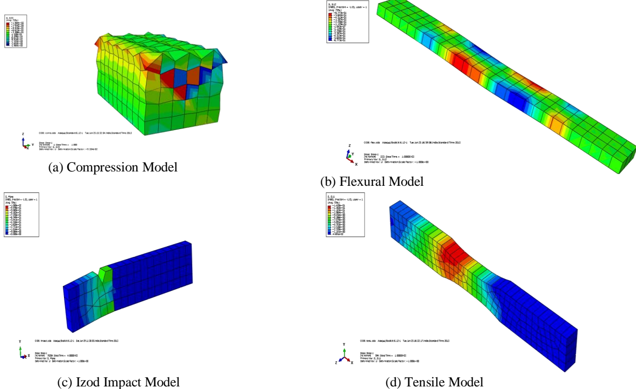
Fig. 4: Compression, Flexural, Izod- Impact and Tensile Failure Models
