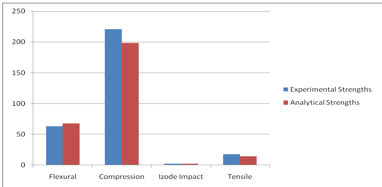
Fig. 5 : Comparisons of Experimental and Analytical Strengths
