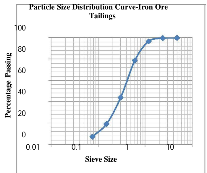
Figure 3: Particle Size Distribution Curve For IOT
