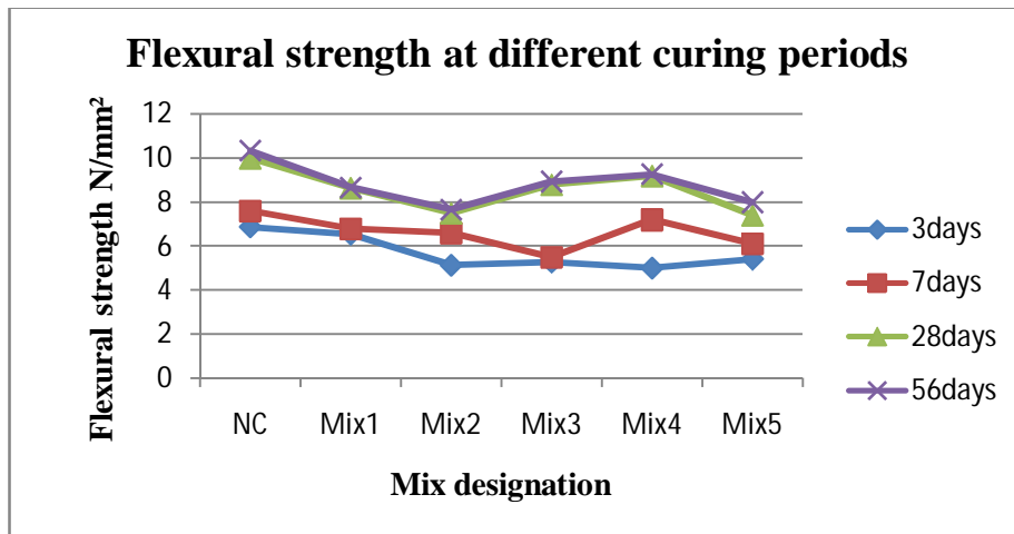
Figure 7: Graph showing Flexural Strength Development of Different Mixes
