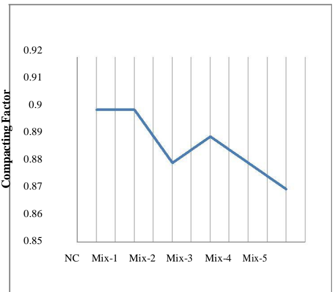
Figure 5: Variability of Compaction Factor
