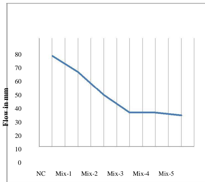
Figure 4: Variability of Slump Value
