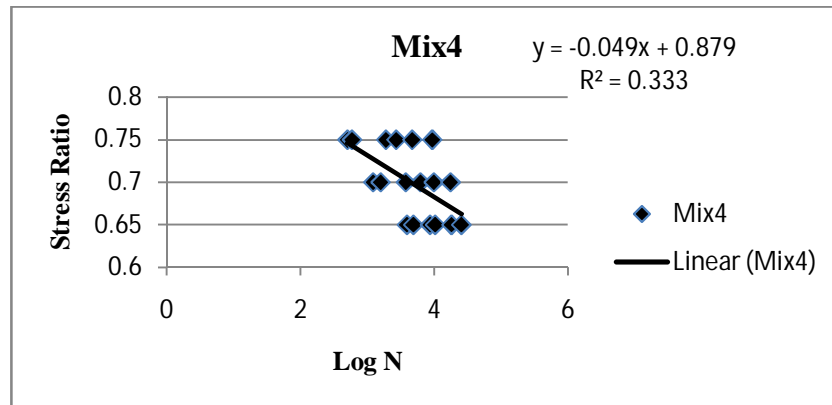
Figure 9: Relationship between Stress Ratio (SR) and number of repetitions N with omitted Values
