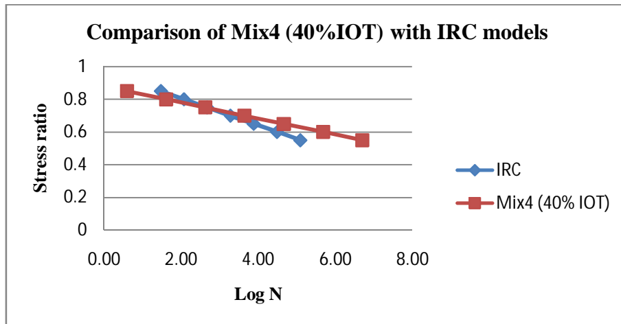
Figure 10: Comparison of Mix4 (40%IOT) with IRC Models
