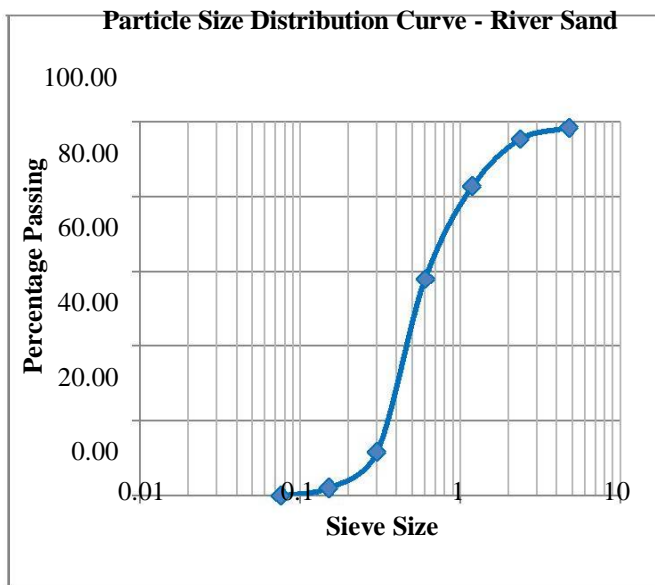
Figure 2: Particle Size Distribution Curve For RiverSand
