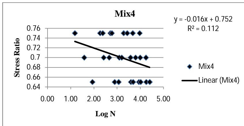
Figure 8: Relationship between Stress Ratio (SR) and number of repetitions N
