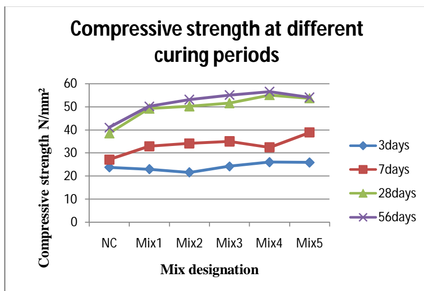
Figure 6: Graph showing Compressive Strength Development of Different Mixes
