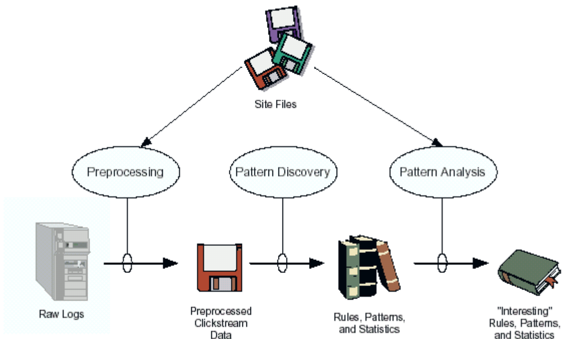
Fig No 01 High Level Web Mining Process
