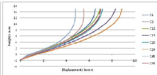
Figure 4.1: Displacements Vs Height for G+4frame without hoarding frame for columns at 33m/sec wind speed. From figure 4.1, it was observed that maximum displacement of 8.869 mm occurs at top storey(i.e. 15m level) for C29 column, which is an interior column. So, it is clear from the values that interior column sharing more load than the end columns.
