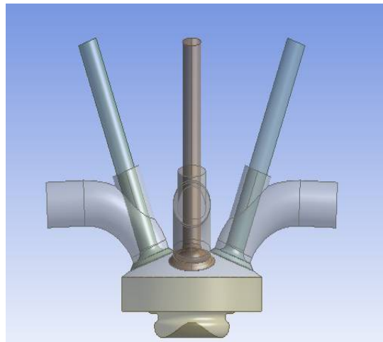
Fig 2: Sector Method geometry for model AVL (TDC to BDC)
