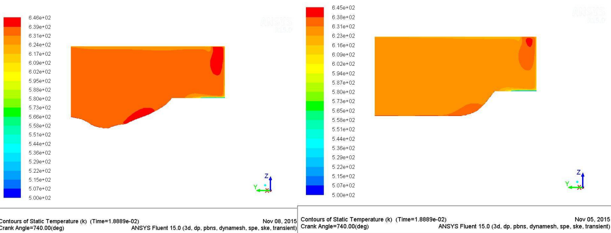
Fig 3: CFD result for model Mitsubishi at CA 740
