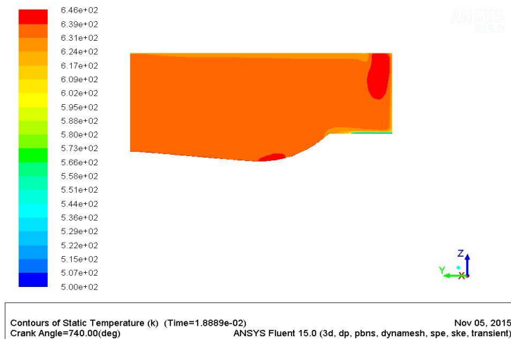
Fig 5: CFD result for model Shallow Hasselman at CA 740
