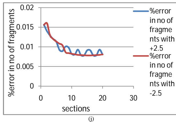
Fig.6. Graphs describing percent error when tolerances are given to ogive radius, left side radius and right side radius:(h) graph representing percent error in angle 2,(i) graph representing percent error in explosive mass,(j)graph representing percent error in number of fragments
