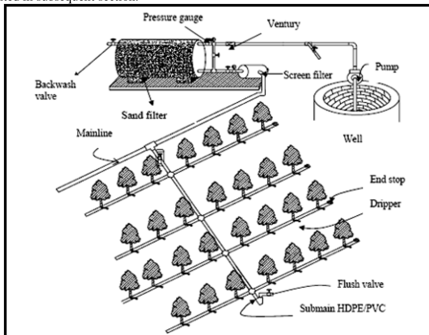
Fig-1:Microirrigation components
