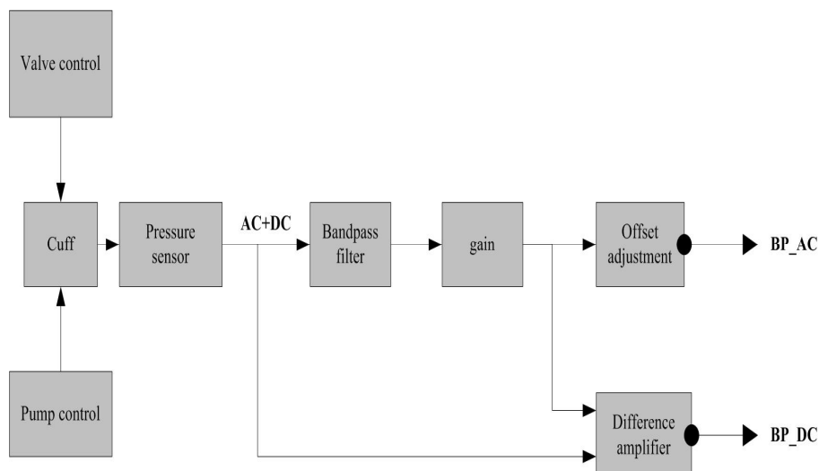
Figure 5: Blood pressure acquisition module
