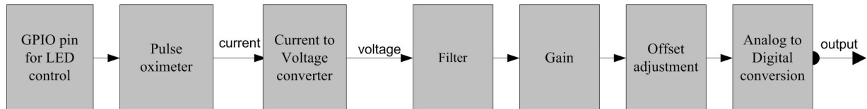
Figure 3: SPO2 acquisition module
