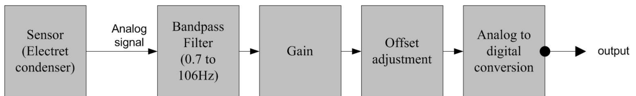
Figure 4: Stetho signal acquisition module
