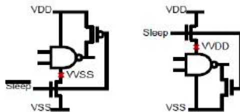
Fig.6 Fine grain power gating
