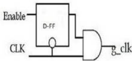
Fig.4 Flip flop based clock gating
