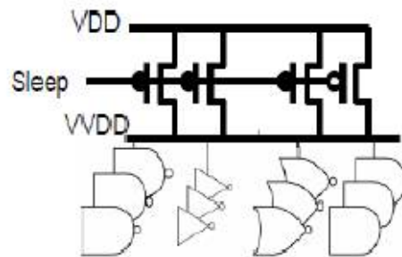
Fig.7 Coarse grain power gating
