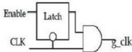
Fig.3 Latch based techniques
