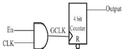
Fig.2 AND based technique
