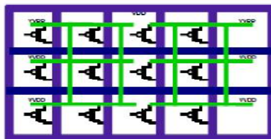
Fig.9 Grid style sleep transistor
