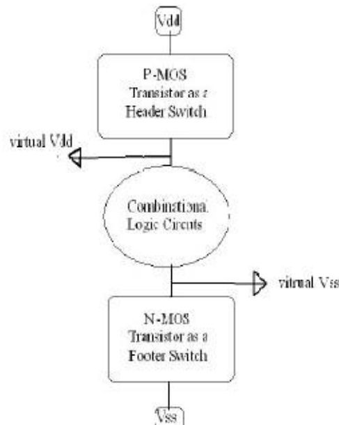
FIG.5 POWER GATING METHODS
