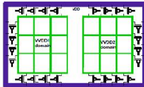
Fig.8 Ring style sleep transistors
