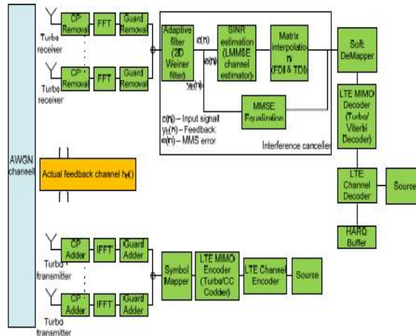
Fig 2: Proposed system model of ICS Repeater without Pilot signal for 3GPP/LTE.
