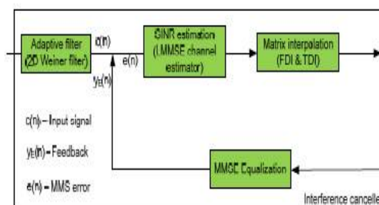
Fig 1: Proposed Iterative model for MIMO receiver
