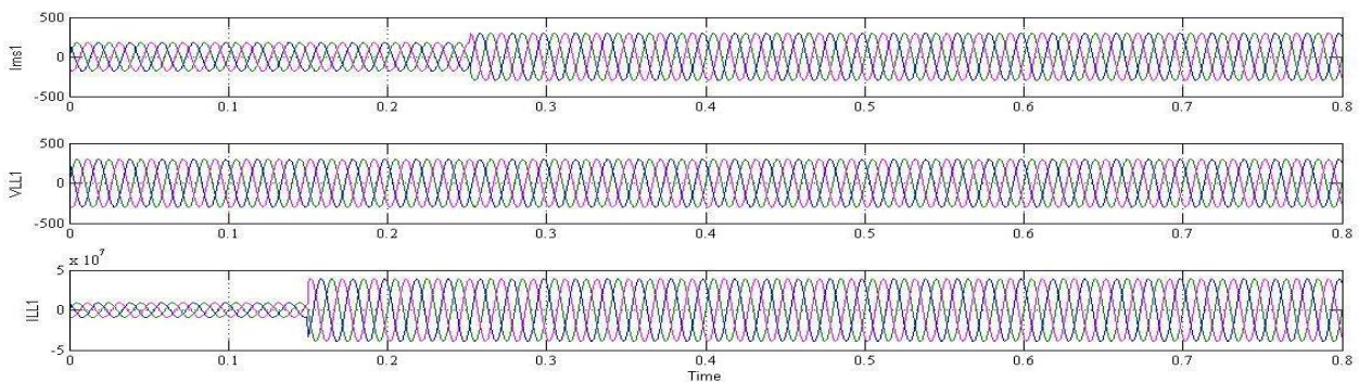
The figure shows the performance of the proposed microgrid comparison of micro turbines, VSI and further connected to the utility grid modeled by synchronous generator. I_{ms1} represents microsource1 output current, V_{LL1} represents local load voltage of microsource1, I_{LL1} represents current flowing into the local load.
