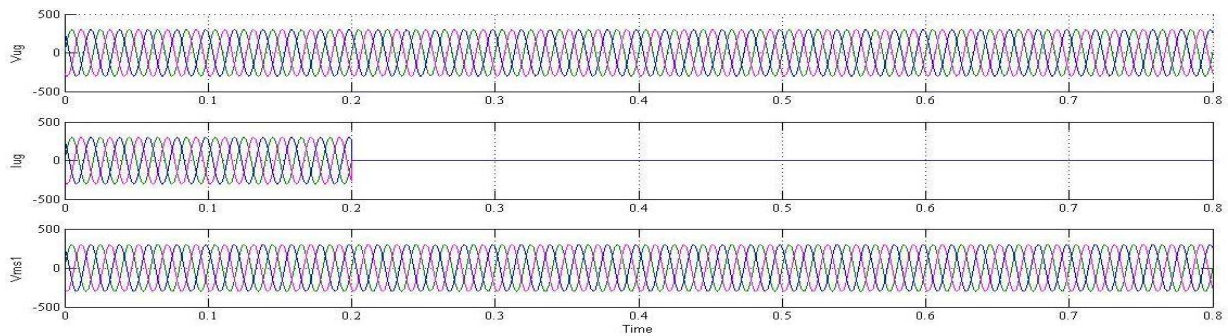
The figure shows the performance of microgrid connected to the utility grid without equal loads on both microsources. V_{UG} represents grid bus voltage, I_{UG} represents grid bus current and V_{ms1} represents microsource1 output voltage.
