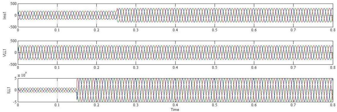
The figure shows the performance of the proposed microgrid comparison of micro turbines, VSI and further connected to the utility grid modeled by synchronous generator. I_{ms1} represents microsource1 output current, V_{LL1} represents local load voltage of microsource1, I_{LL1} represents current flowing into the local load.
