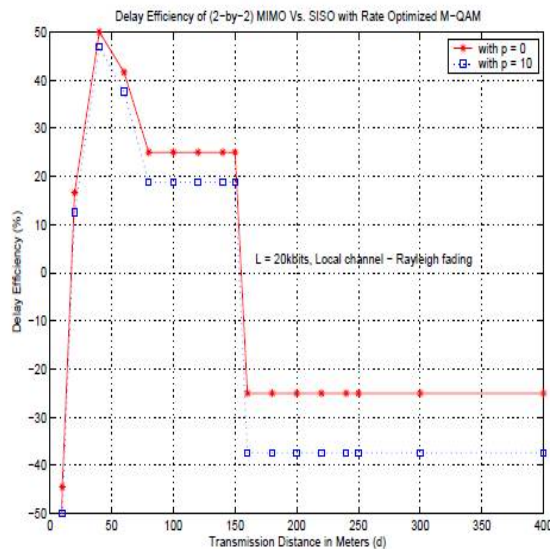
Fig 2: Delay Efficiencies of Virtual 2 \times 2 MIMO and SISO with Rate Optimized M-QAM
