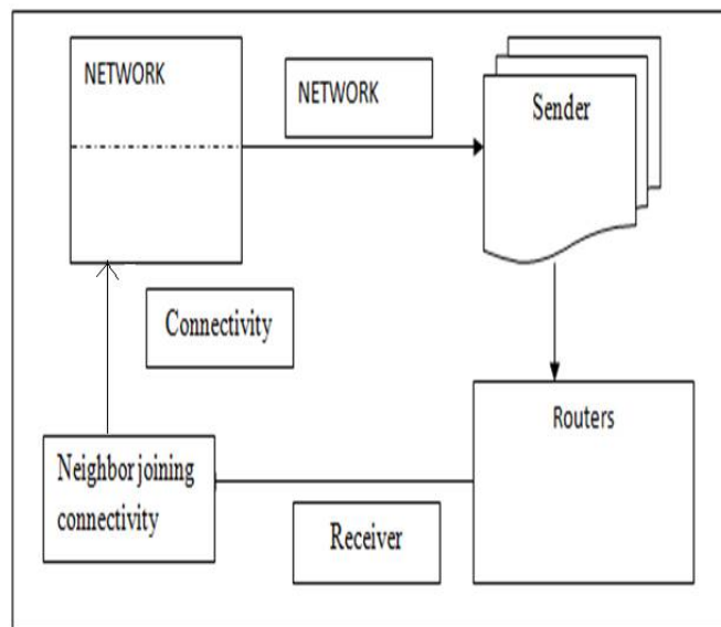
Fig 1: System Architecture
