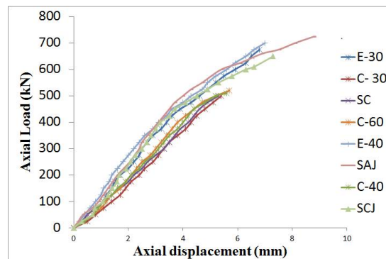
Fig. 3. Load- displacement curve
