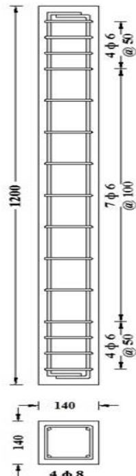
Fig. 1. Reinforcement detailing of column specimens
