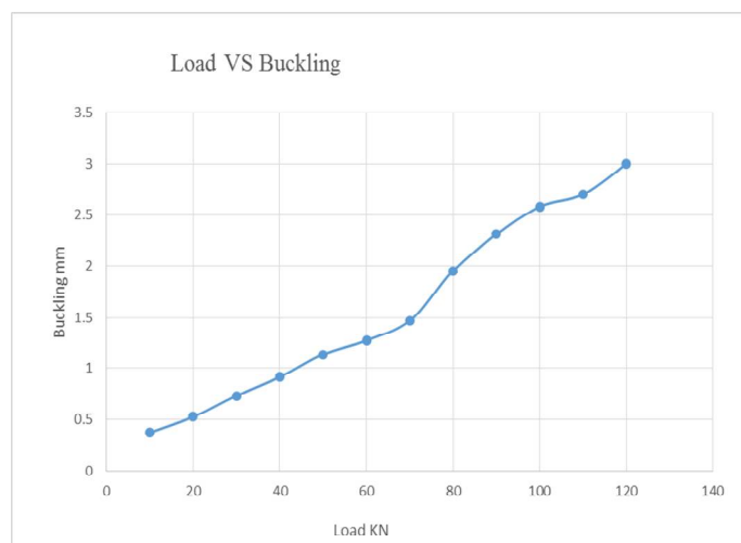
Figure 7. Load Vs Buckling graph of circular column with bar reinforcement
