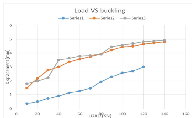
Figure 10. Comparison of all the columns
