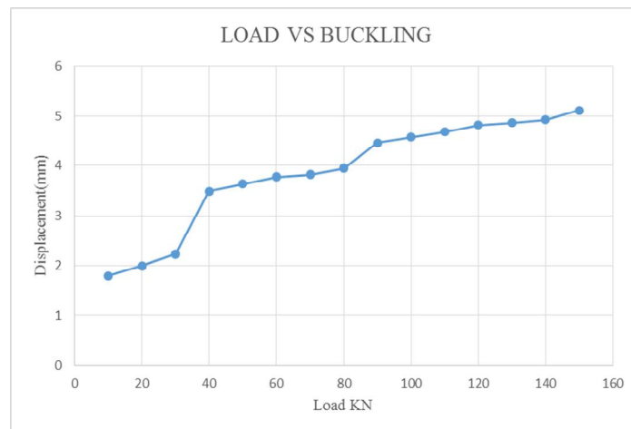
Figure 9. Load Vs Buckling graph of FRC column with hollow GI pipe
