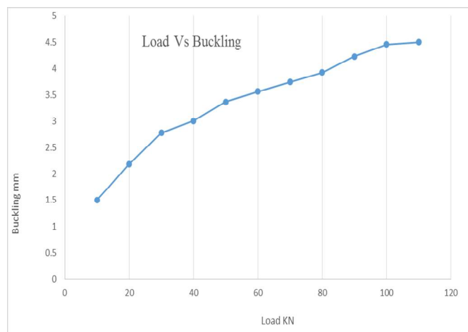
Figure 8. Load Vs Buckling graph of circular column in with GI pipe
