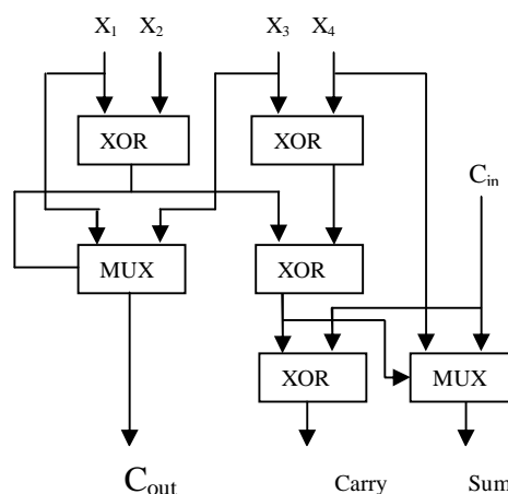
Figure 2(b): 4:2 Compressors using XOR Gate
