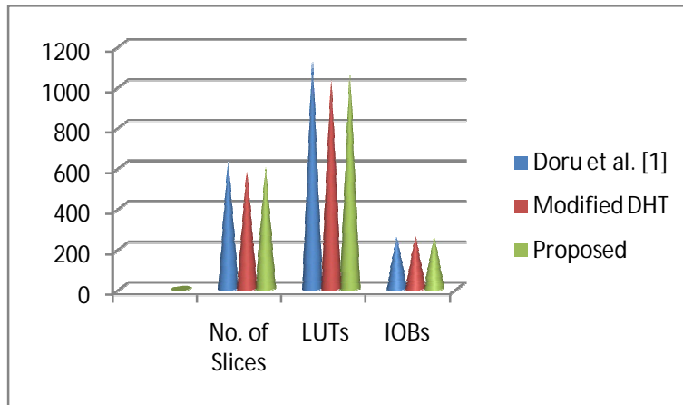
Figure 7: Show the bar graph of 8-bit DHT with word length 16
