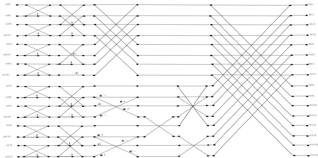
Figure 5: 16-point DHT Butterfly
