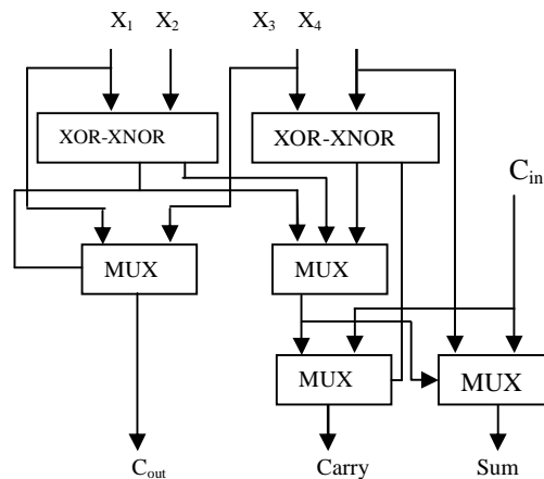
Figure 2(c): 4:2 Compressors using XOR-XNOR Gate
