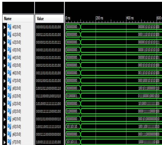
Figure 8: Output Waveform of 8-bit DHT with word length 16
