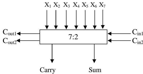
Figure 3: Block Diagram of 7:2 Compressors
