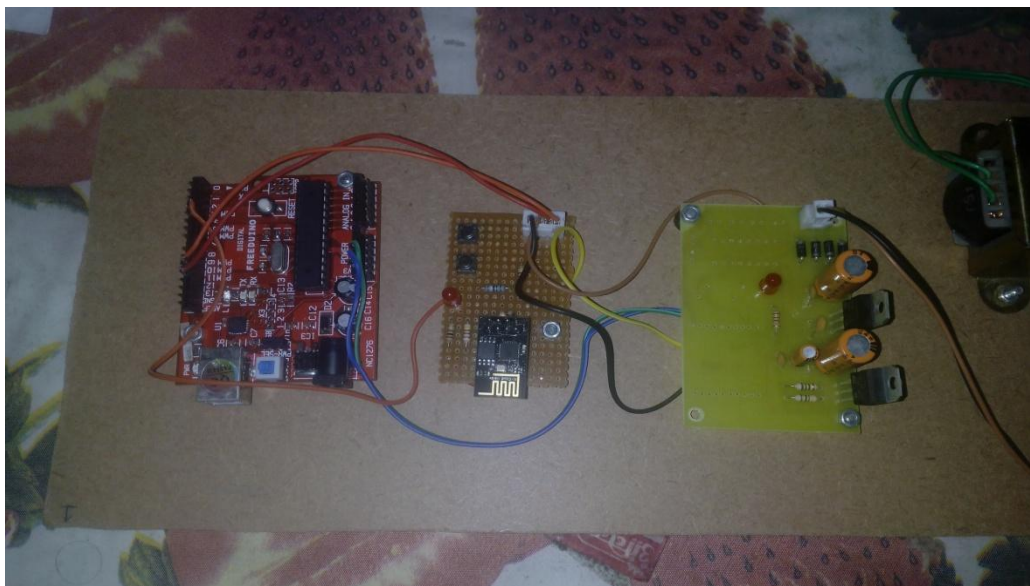
Fig No 02 System Design
