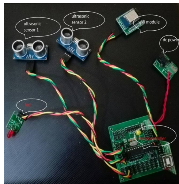
Fig.9 (b) Actual setup of Non Contact Liquid Monitoring System
