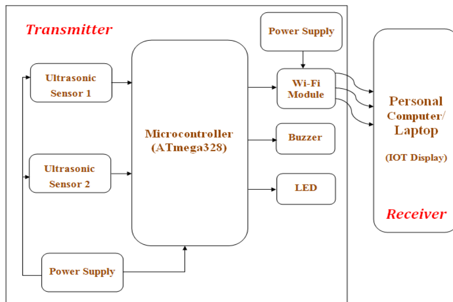
Fig.2. Block diagram of Non Contact Liquid Monitoring System
