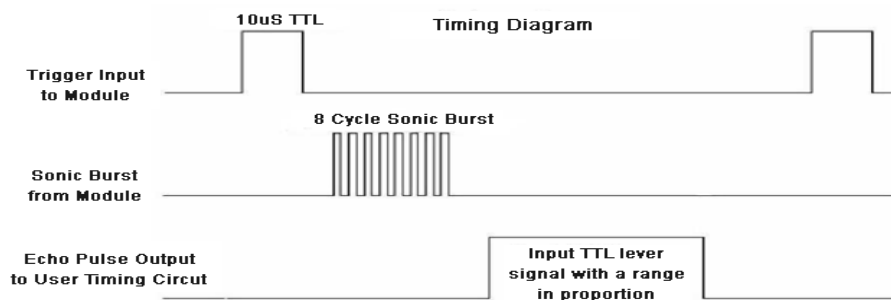
Fig.5.The HC-SR04 timing diagram
