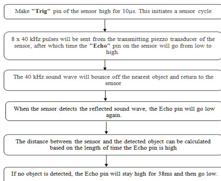
Fig.6. Basic algorithm in distance measuring using the Ultrasonic sensor
