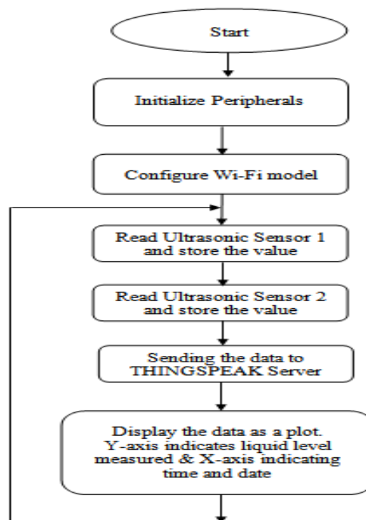
Fig.10. Flowchart for the Non Contact Liquid Monitoring System
