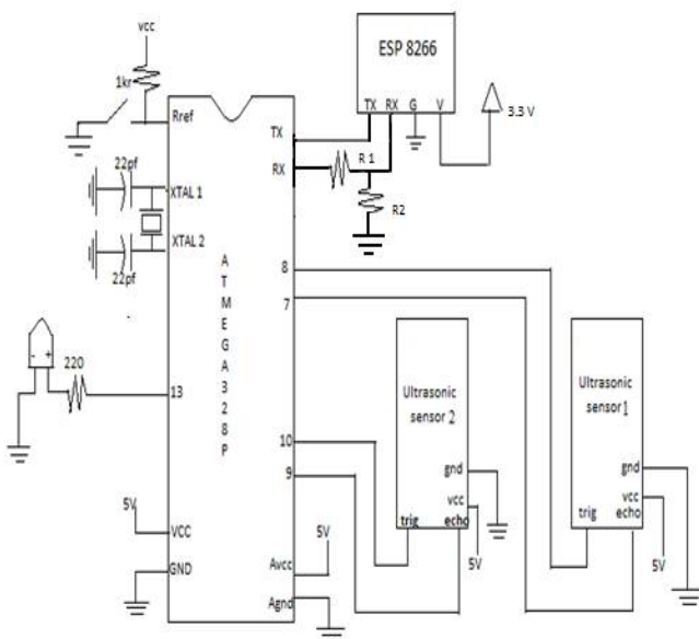
Fig.9 (a) Circuit diagram of Non Contact Liquid Monitoring System
