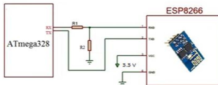
Fig.7. Connection between Wi-Fi module and Microcontroller
