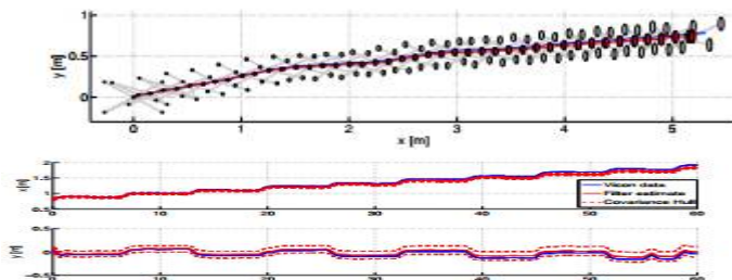
Fig. 2. 2D view of a 5 m trotting sequence in simulation. Blue: ground-truth body trajectory. Red ellipses: successive position estimates of the robot's main body. Grey ellipses: estimates of the foothold positions. In both cases the ellipses are scaled depending on the corresponding standard deviation ( 1\sigma ). The position error at the end amounts to less than 5% of the traveled distance.
