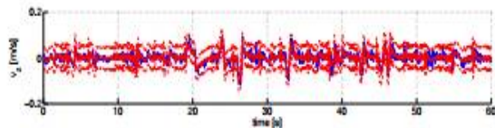
Fig. 4. Comparison between estimated velocity and the motion capture system's numerical position derivatives. All three velocity estimates are fully observable and consequently can be tracked very accurately. The resulting RMS error values are 0.0111 m/s, 0.0153 m/s and 0.0126 m/s.
