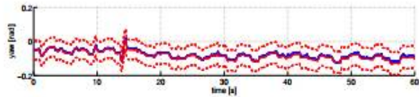
Fig. 5. Comparison between estimated roll, pitch and yaw angle and the motion capture system's orientation outputs. Roll and pitch angle are fully observable and the filter produces very precise corresponding estimates, with angular error RMS of less than 0.5 deg (0.0088 rad and 0.0073 rad). The yaw angle drift is almost unnoticeable.
