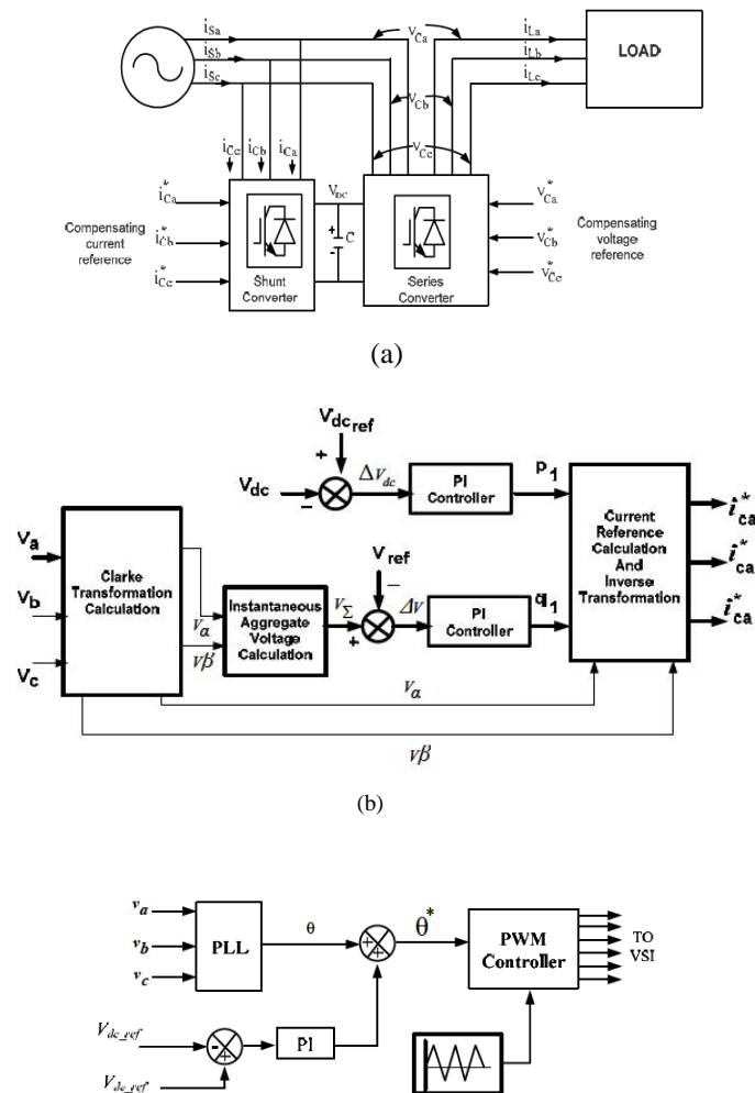
Fig. 5 (a) Shunt current and voltage compensation (b) Control block of shunt current compensation. (c) Control Block of Series Converter
