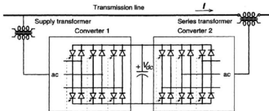
a. Basic UPFC conventional diagram
