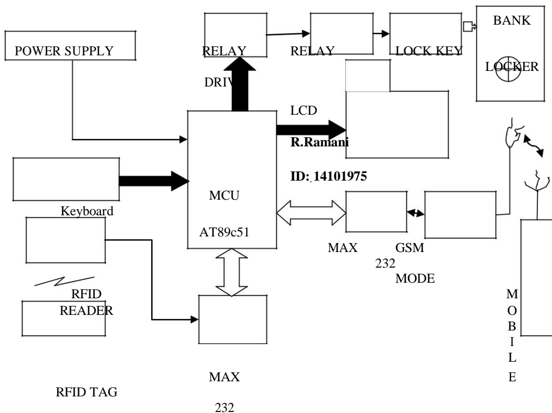
Figure3. Block diagram of Bank locker system based on RFID and GSM technology
