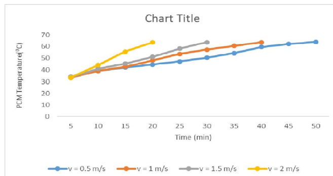
Fig. 4 Variation of PCM Temperature with time during Charging at heat input 1000 W
