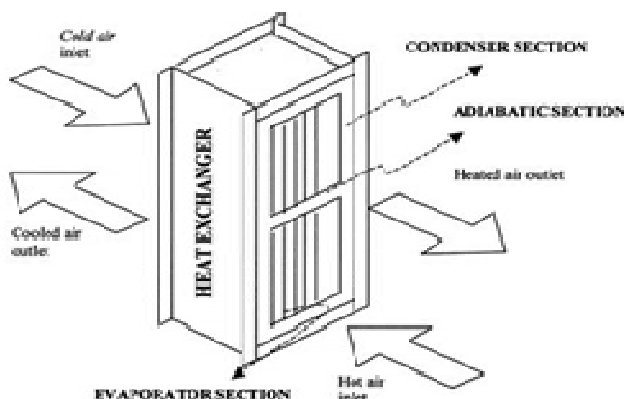
Fig. 1 Schematic of the PCM air heat exchanger.
