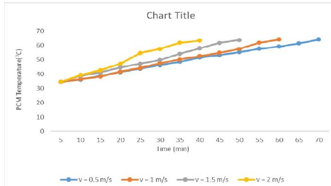
Fig. 3 Variation of PCM Temperature with time during Charging at heat input 750 W
