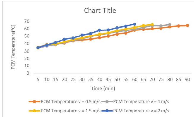
Fig. 2 Variation of PCM Temperature with time during Charging at heat input 500 W
