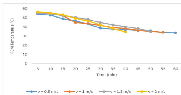
Fig. 7 Variation of cold air outlet temperature with time during Discharging at heat input 1000w
