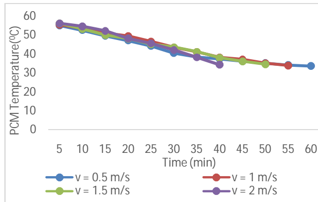
Fig. 5 Variation of cold air outlet temperature with time during Discharging at heat input 500 W
