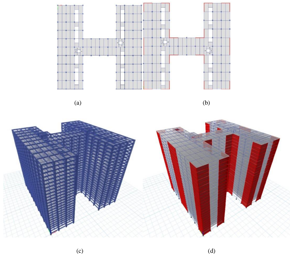
Fig. 1. Model details (a) Plan view of H-shape structure without shear wall (b) Plan view of H-shape structure with shear wall (c) 3D view of H-shape structure without shear wall (d) 3D view of H-shape structure with shear wall
