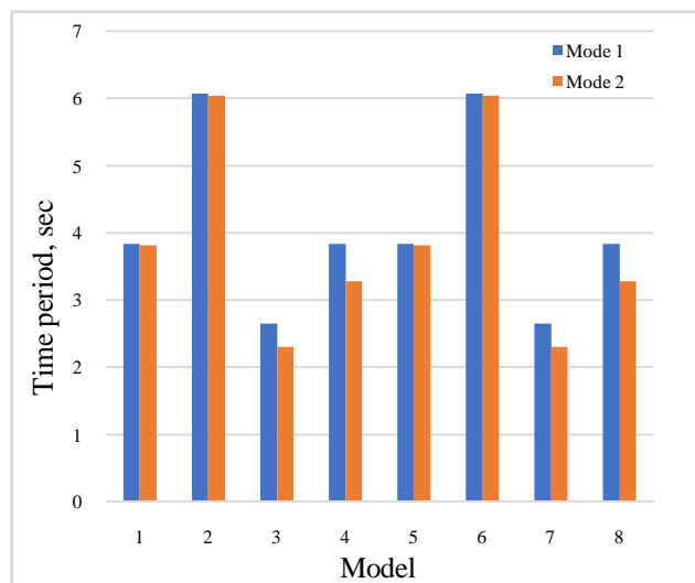
Fig. 6. Time period
