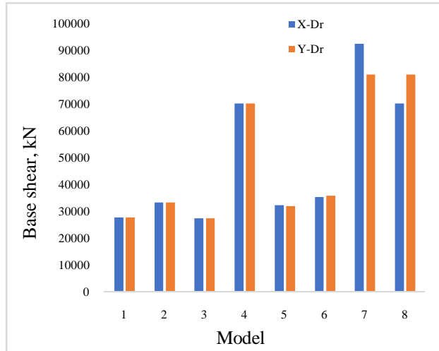
Fig. 7. Base shear
