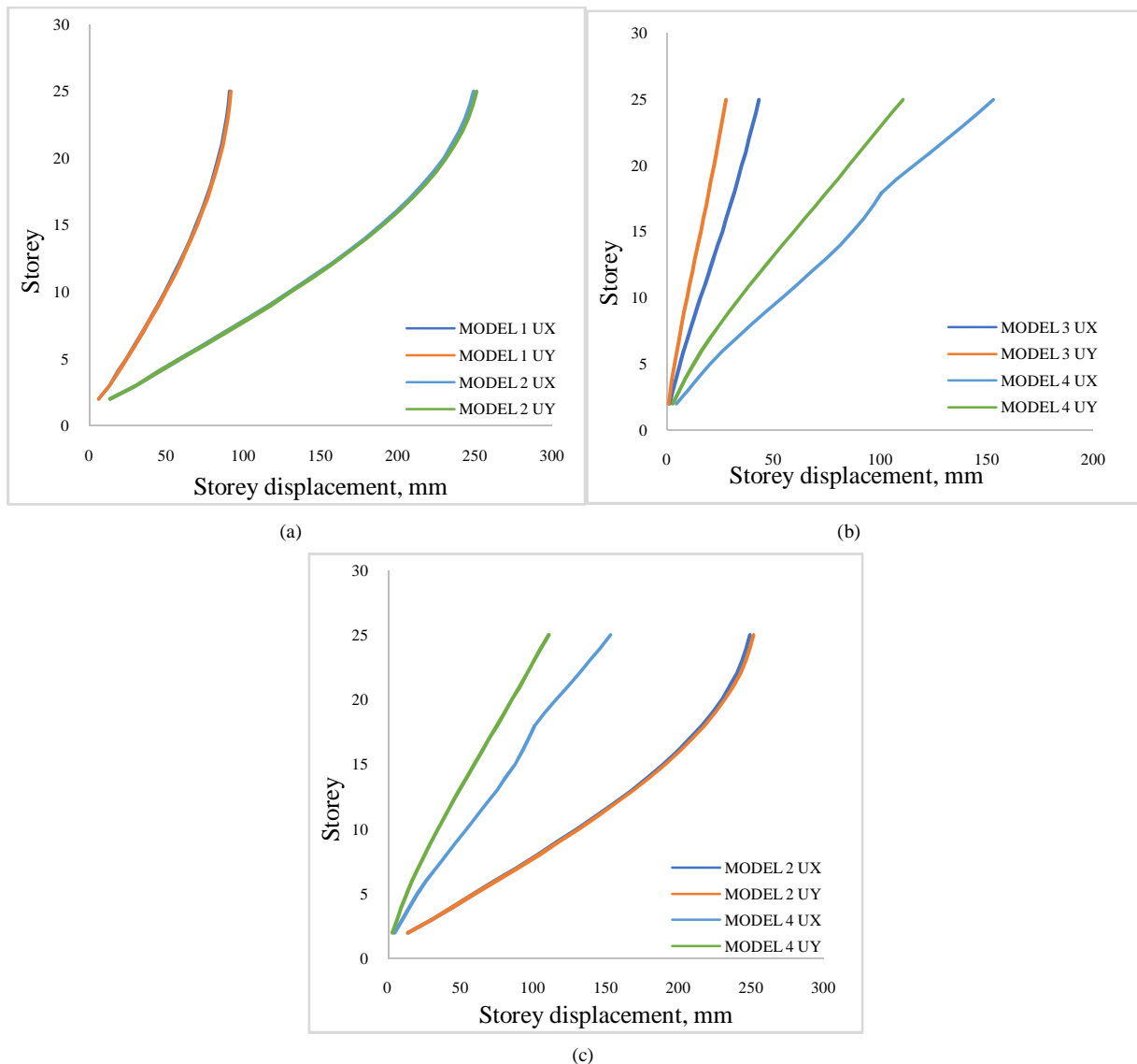
Fig. 2. Storey displacements (a) Model M1 and M2 (b) Model M3 and M4 (c) Model M2 and M4
