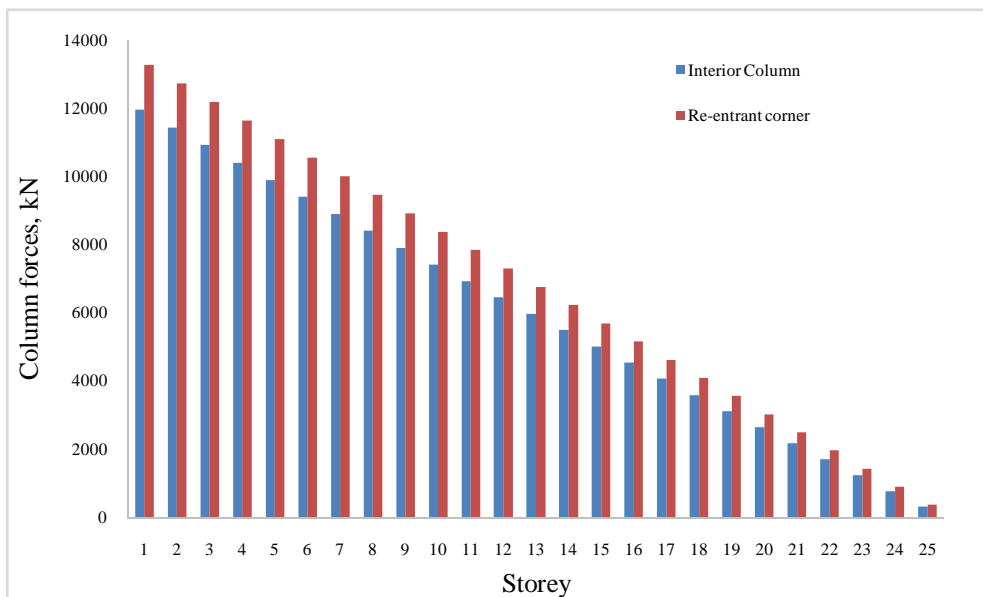
Fig. 8. Column forces
