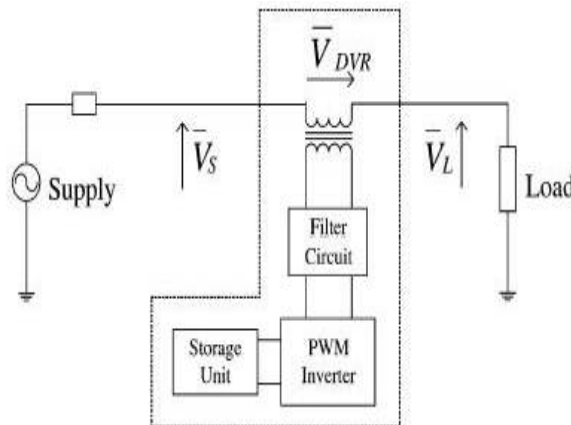
Fig.1 Schematic diagram of DVR
