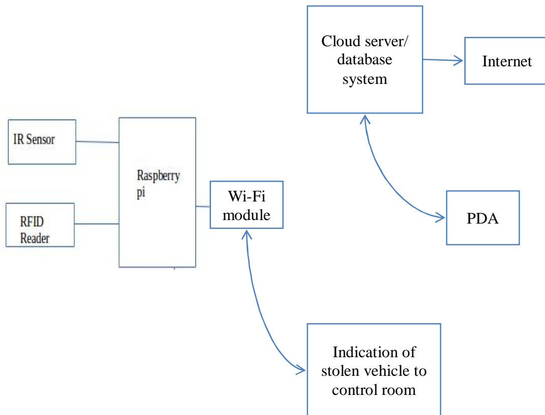
Fig.1 – Cloud based smart vehicle and anti-theft system using IOT
