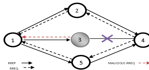
Fig.3 Black Hole Attack
