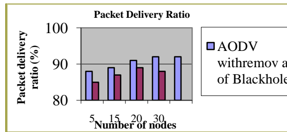
Fig.7 Packet Delivery Ratio
