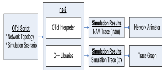
Fig.6. Network Simulator-2
