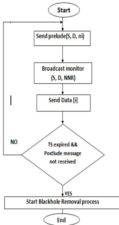
Fig.4. Detection of Black Hole Activity
