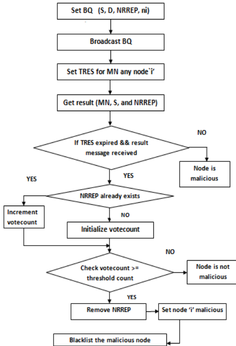
Fig.5 Flow Chart for Black Hole Removal
