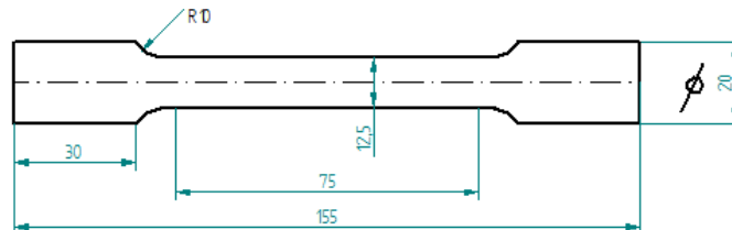
Fig 2. ASTM standard for dimensioning tensile specimen
