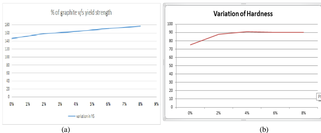
Fig 9. Variation of yield strength and hardness of the tested specimen with variation in graphite percentage
