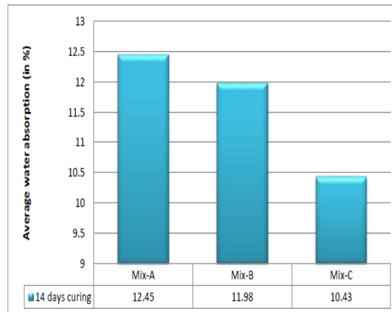
Graph.3. Average water absorption of all mix proportions
