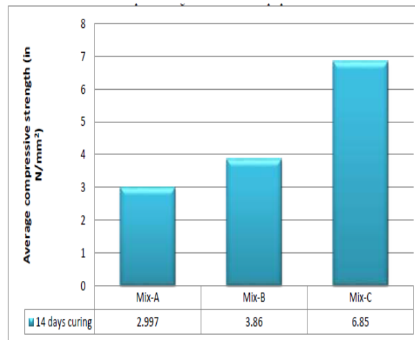
Graph.2. Average compressive strength of all mix proportions
