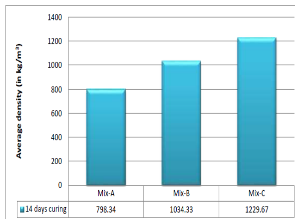
Graph.1. Average densities of all mix proportions
