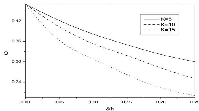
Fig. 2: Flow rate for different values of permeability parameter K
