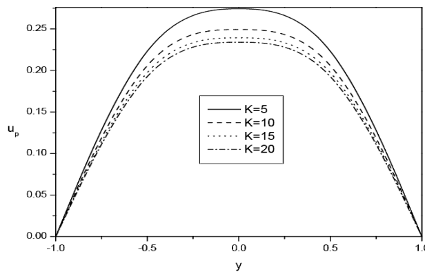
Fig. 1: Variation of u with permeability parameter K
