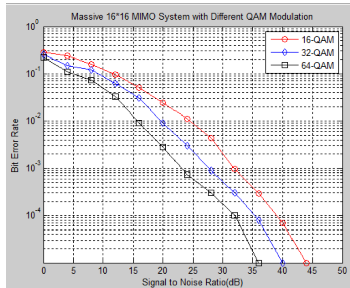
Figure 4: BER vs SNR for Massive 16×16 System with QR-RLS based Channel Estimation Technique
