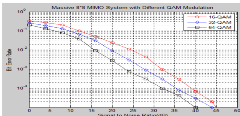
Figure 3: BER vs SNR for Massive 8 \times 8 System with QR-RLS based Channel Estimation Technique
