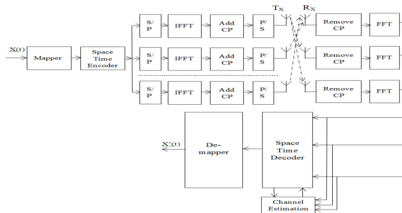
Figure 2: Massive MIMO System Models with Channel Estimation Technique
