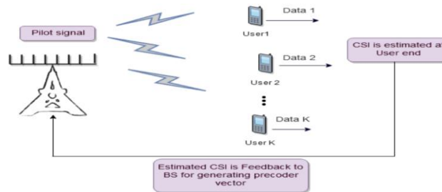
Figure 1: Downlink transmission in an FDD Massive MIMO system
