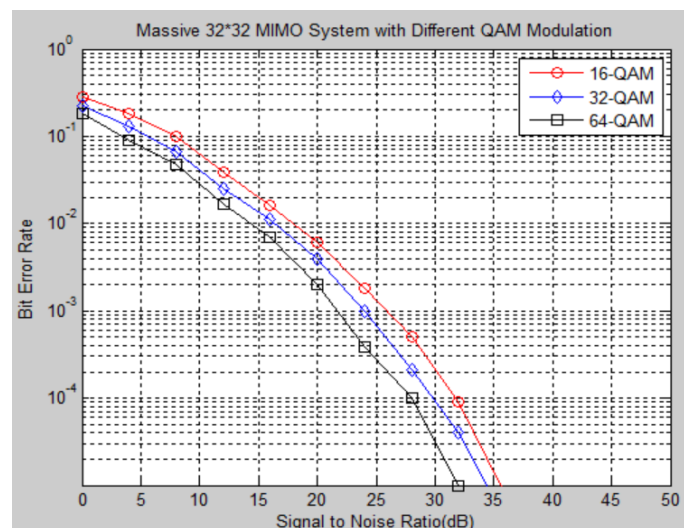
Figure 5: BER vs SNR for Massive 32×32 System with QR-RLS based Channel Estimation Technique
