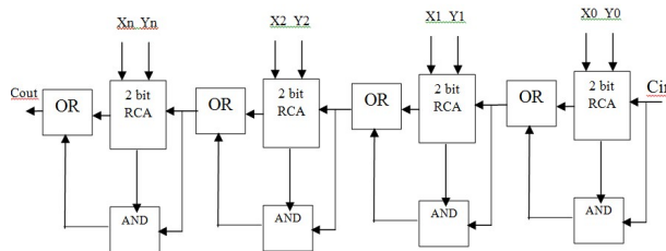
Figure 5: Carry Skip Adder
