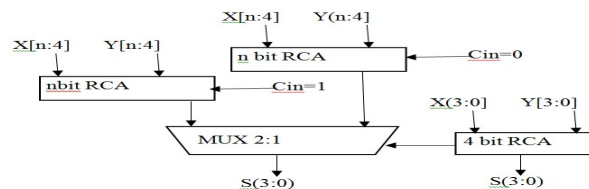
Figure 6: Carry Select Adder
