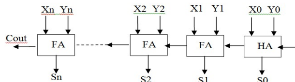
Figure 3: Parallel Adder (n=7 for SPFP and n=10 for DPFP)
