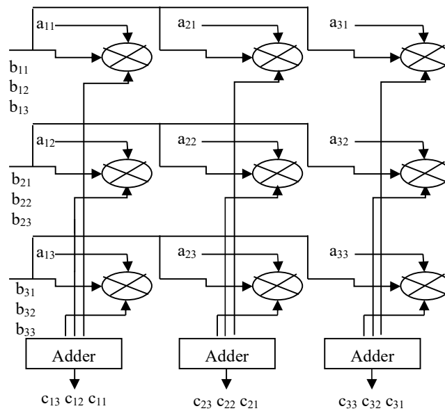
Figure 8: Proposed PPI – MO Design for n = 3
