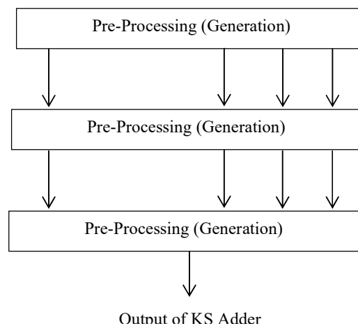
Figure 7: Block Diagram of Kogge Stone Adder
