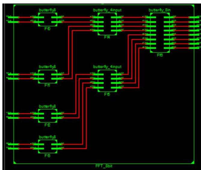
Figure 10: RTL View of DIT 8-point DIT-FFT algorithm
