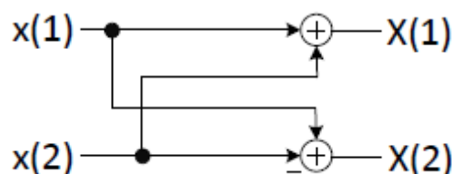
Figure 6: Radix-2 Butterfly
