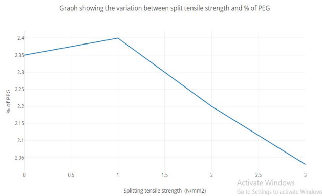
Fig 3 Graph showing the variation between split tensile strength and % of PVA of sample(a)
