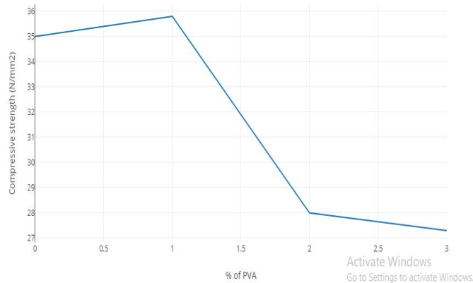
Fig 2. Graph Showing the variation between compressive strength and % of PVA of sample (b)
