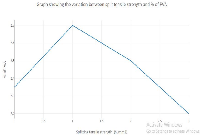
Fig 4 Graph showing the variation between split tensile strength and % of PVA of sample(b)
