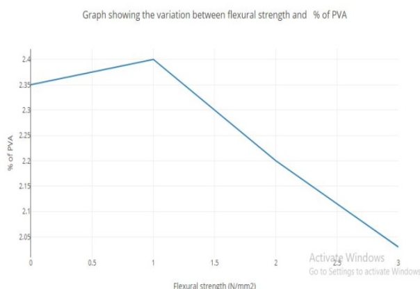
Fig 6 Graph showing the variation between flexural strength and % of PVA.of Sample (b)
