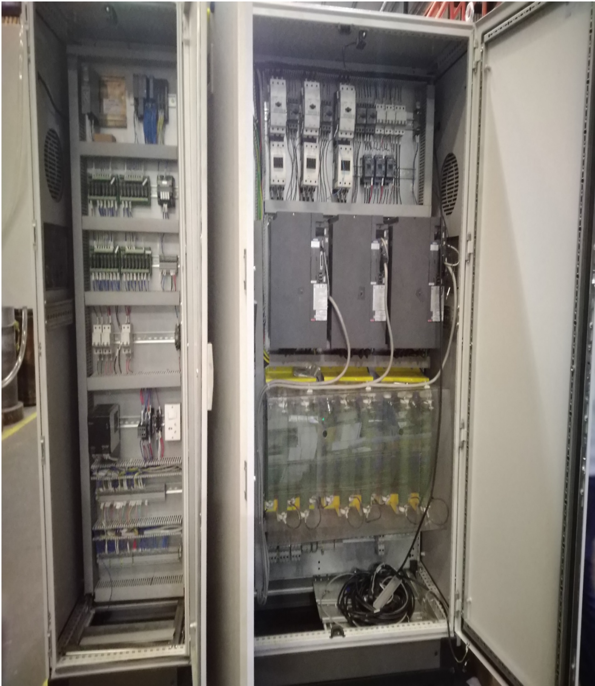
Fig3.1 hardware of control panel
