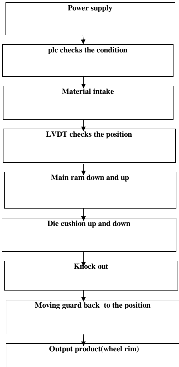
Fig: 4.2 flow chart for whole process
