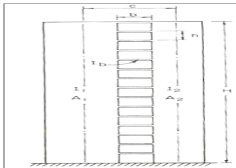
Fig 2.6.1 Coupled shear walls
