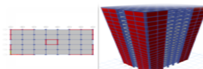
Fig 5.1.2 Shear wall at corner and lift building
