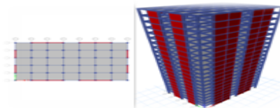
Fig 5.1.3 Shear wall at alternative positions
