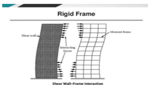
Fig 3.6.2 Shear wall - Frame interaction
