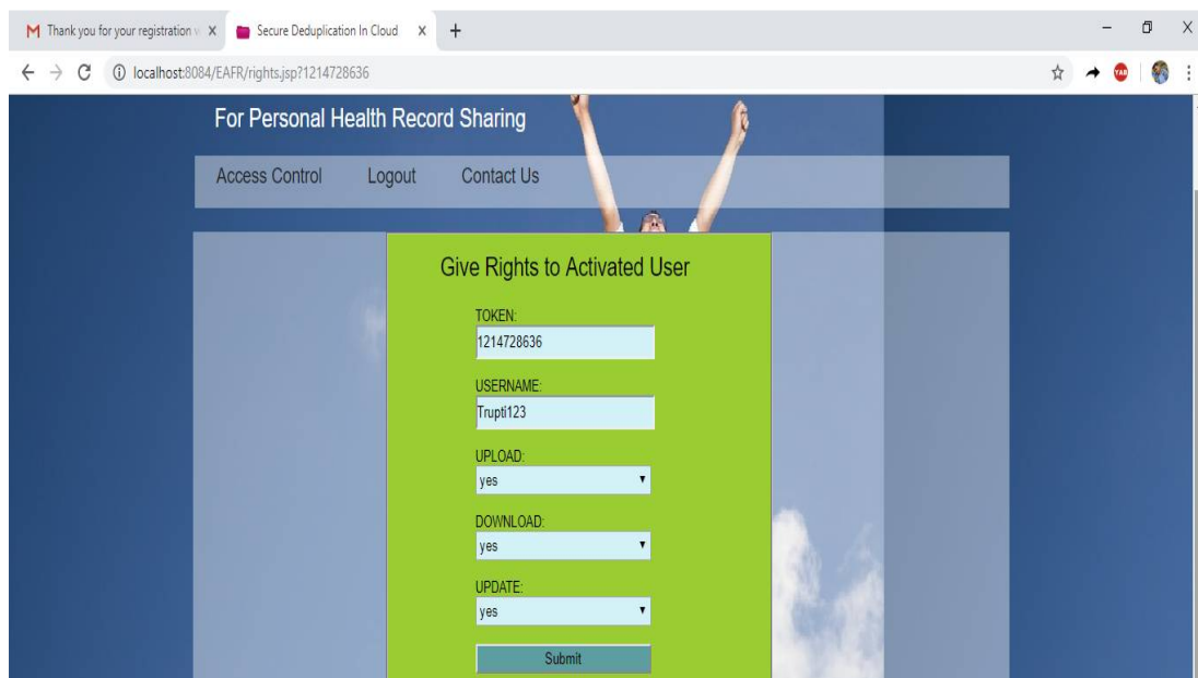
Fig. 3: User Activation
