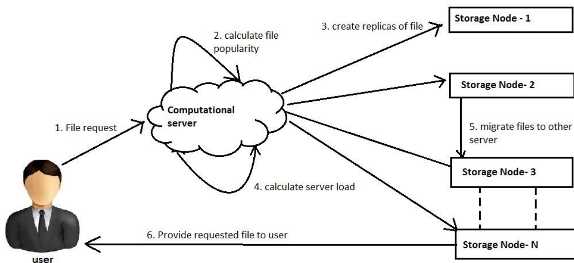
Fig. 1: System architecture
