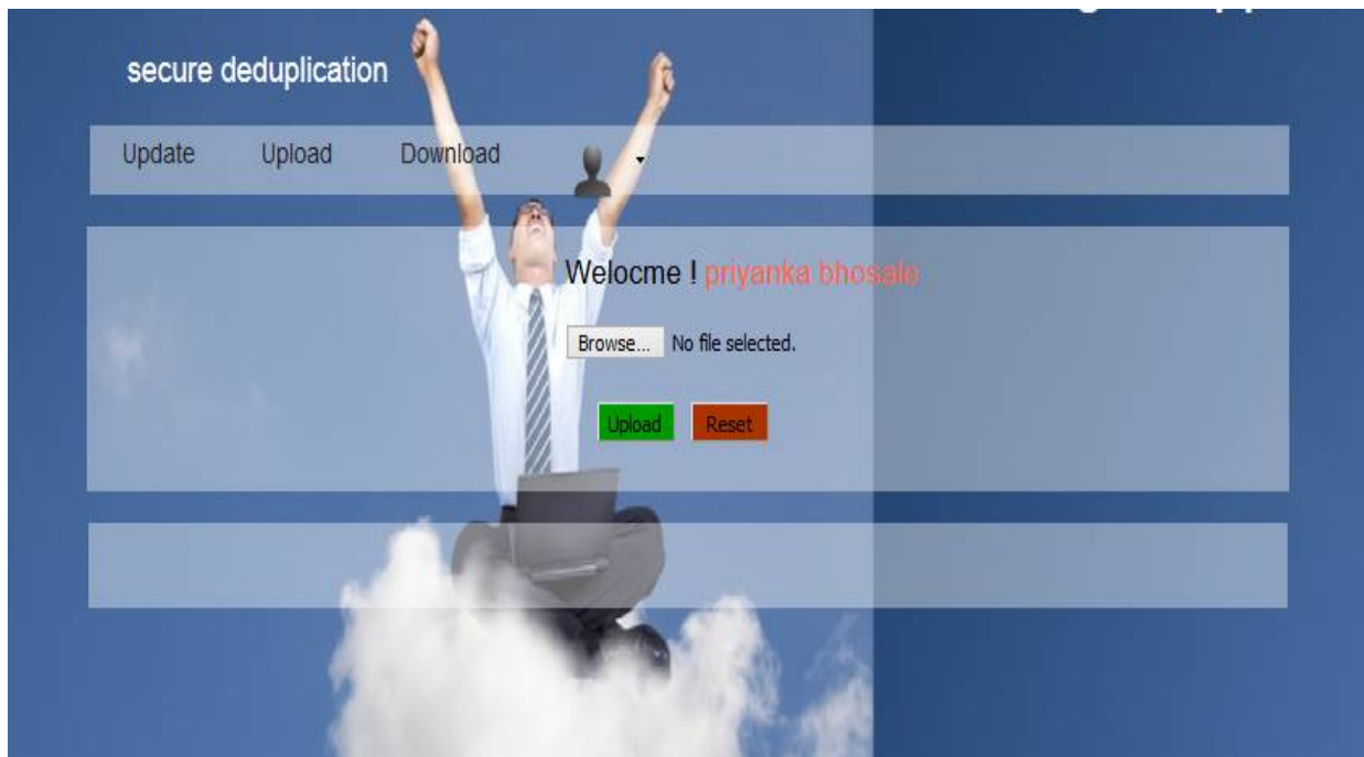
Fig. 4: Upload Files
