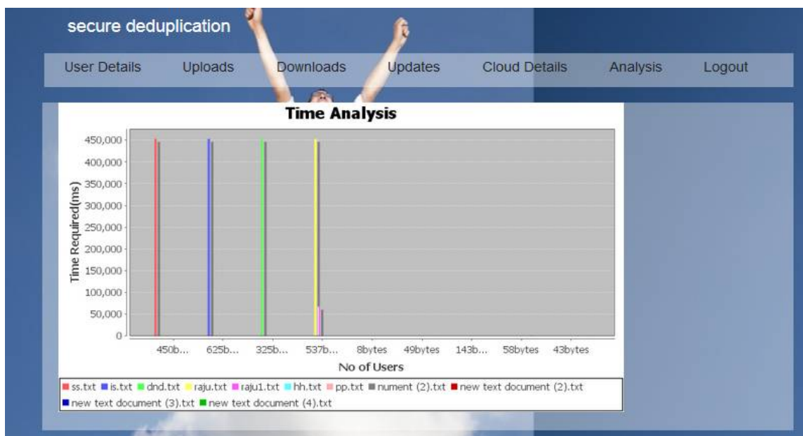
Fig. 5: Time Analysis
