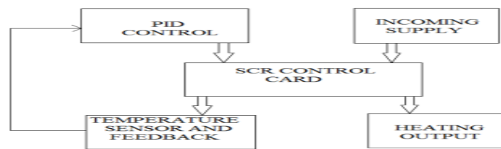
Figure 1. block diagram of pid based thyristor
