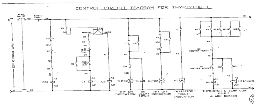
Figure 2. circuit diagram of thyristor
