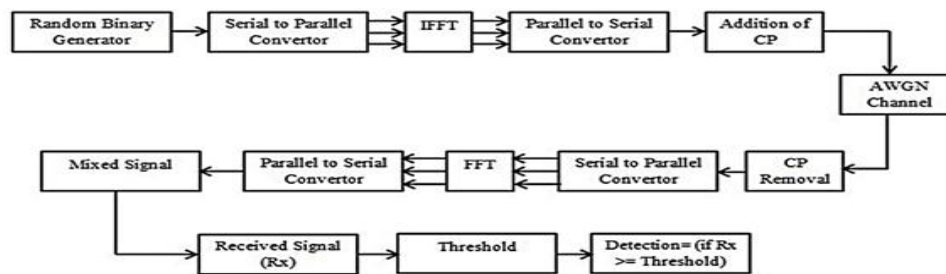
Fig. 2: Proposed MIMO-OFDM System using Matched Filter Detection Technique
