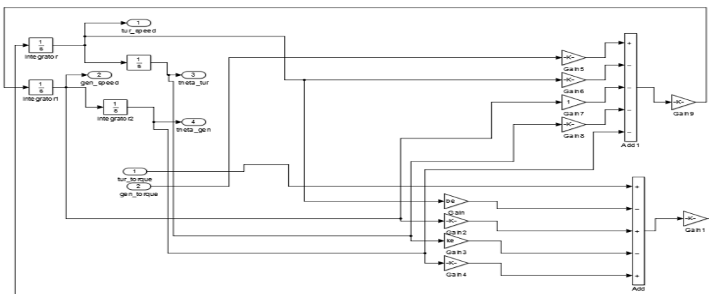
Figure 3.3: Two mass drive train system Matlab model
