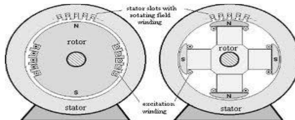
Figure 2.4: Cross section of a synchronous generator
