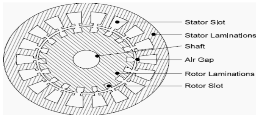
Figure 2.3: Cross-section of asynchronous generator with squirrel cage rotor( http://electrical-engineering-portal.com )
