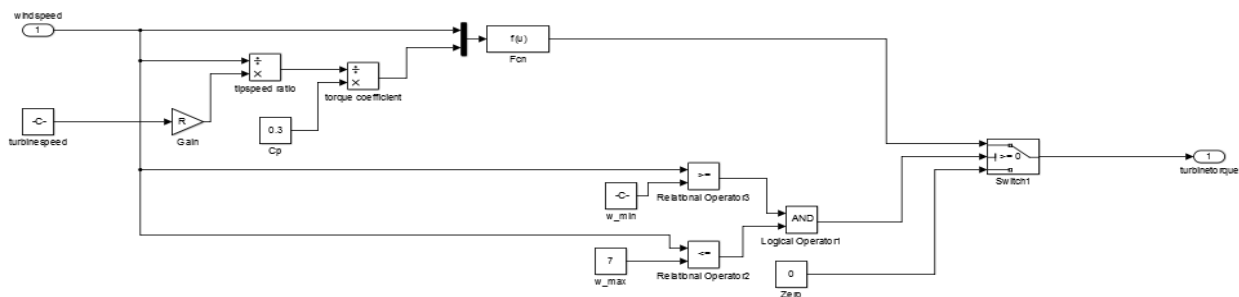
Figure 3.1: Wind turbine subsystem Matlab model
