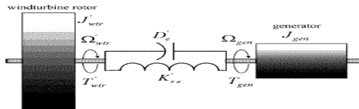
Figure 3.2: Two mass drive train system (Vlastimil Santin, 2011).
