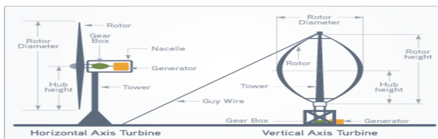
Figure 2.1: wind turbine types Source: http://www.hillcountrywindpower.com/wind-basics.php
