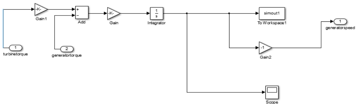
Figure 3.5: One mass drive train Matlab system
