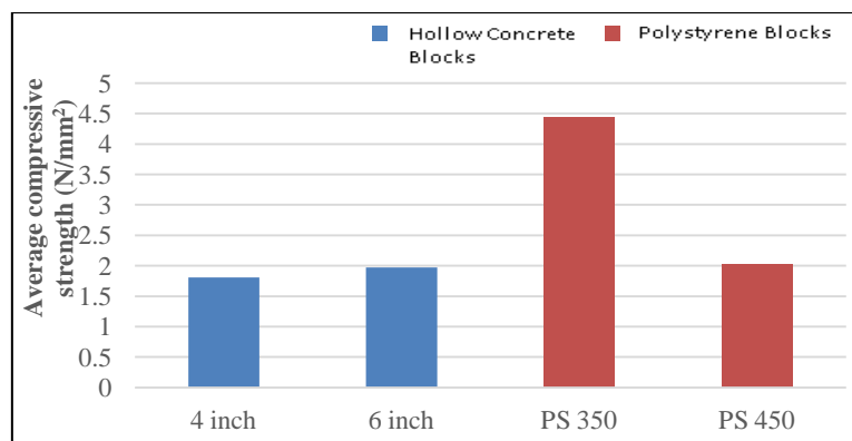
Fig 10 Graph showing average compressive strength of Hollow concrete blocks and Polystyrene blocks
