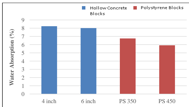
Fig 8. Graph showing Average Water absorption Percentage of Hollow concrete blocks and Polystyrene blocks
