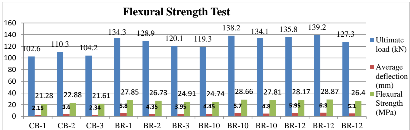
Fig : 6.1 Graphical representation of flexure test results
