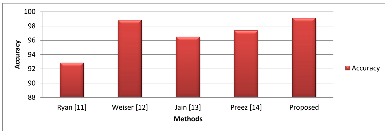
Figure 3 :Selfie detection accuracy of proposed system vs. various existing approaches
