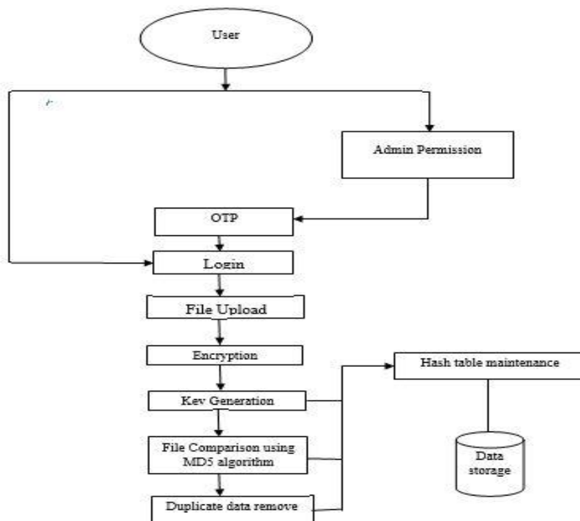
FIGURE 1: SYSTEM ARCHITECTURE
