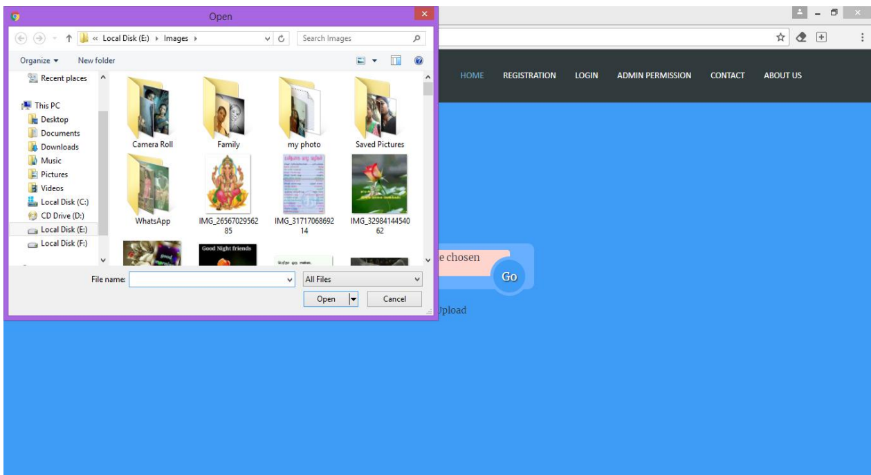
FIGURE 4: FILE UPLOADING
