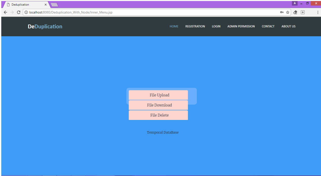
FIGURE 3: FILE UPLOAD
