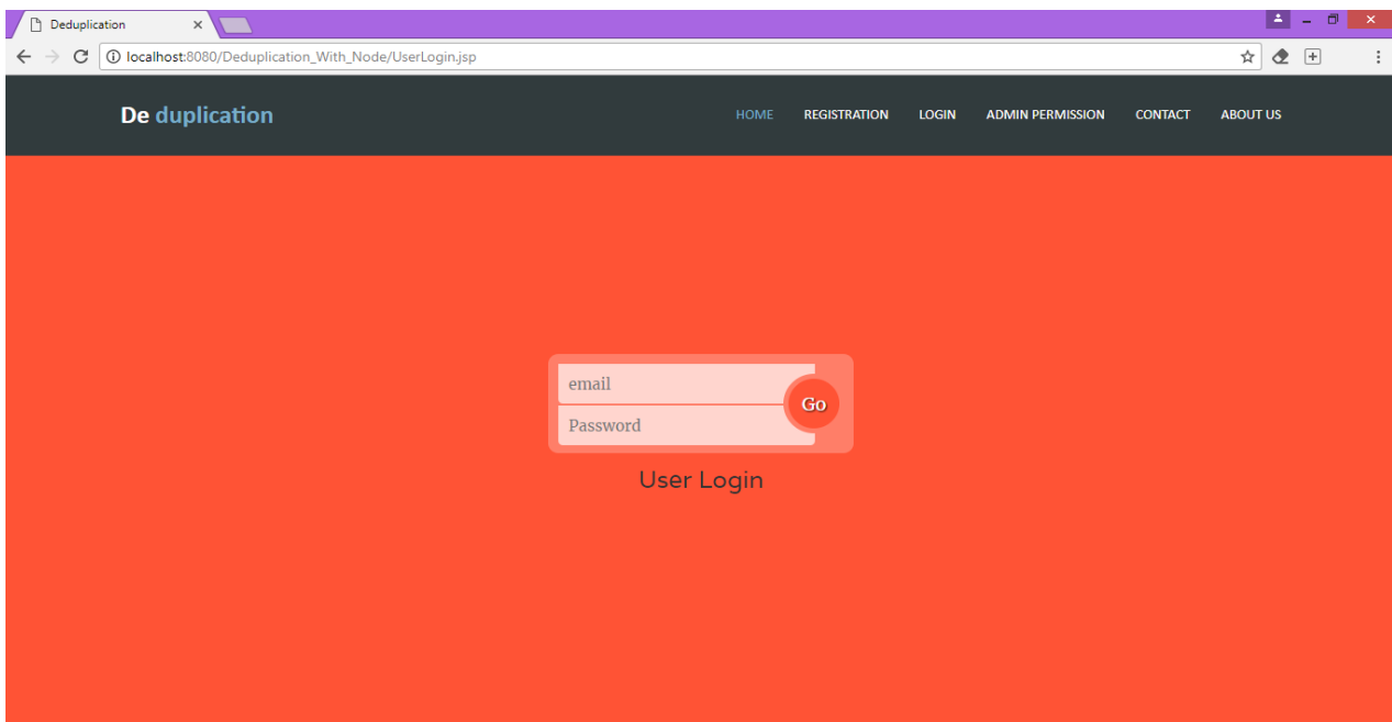
FIGURE 2 : USER LOGIN
