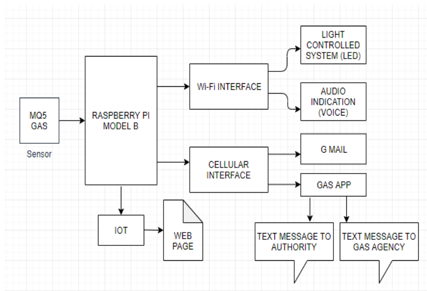
Fig 1: LPG Gas Leakage Sensing and Alerting System
