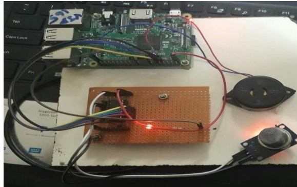
Fig 3: Overall Hardware Setup.
