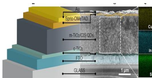
Figure 3 SEM image of the solar cell after annealing at 400deg cell
