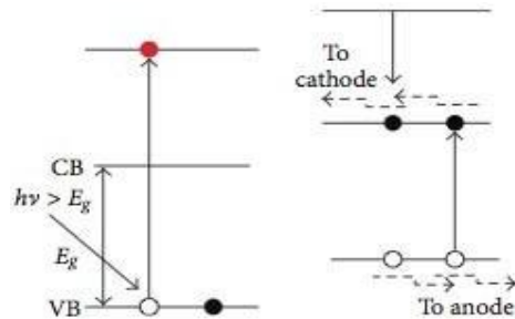
Figure 2b Mechanism of Impact ionization
