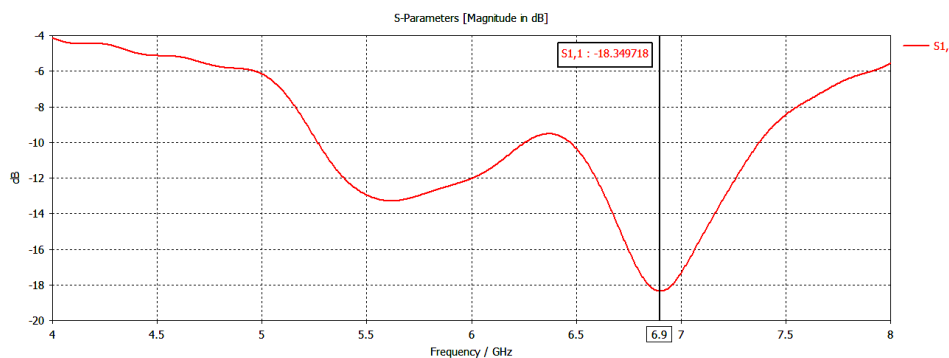
Figure 4: Return loss
