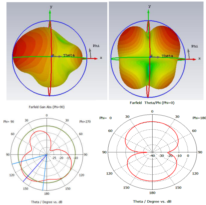
Figure 8: Radiation pattern
