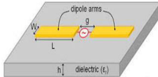
Figure 1: Microstrip Antenna
