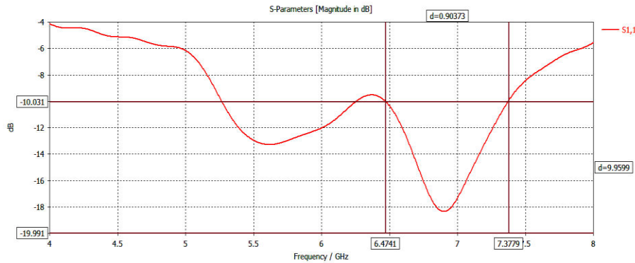
Figure 5: Bandwidth
