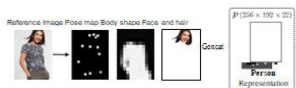
Figure 3: A clothing-agnostic person representation.
